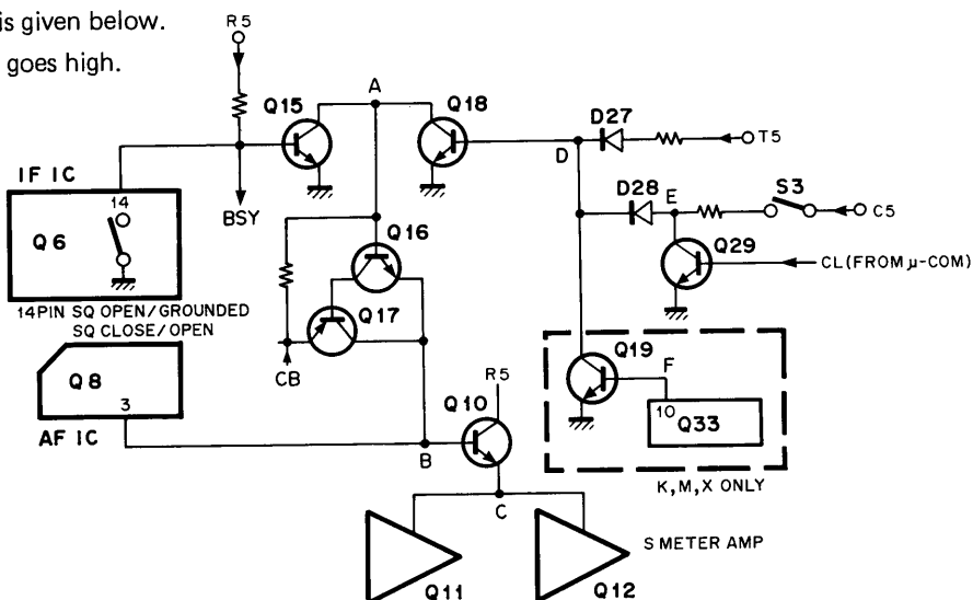
Fig. 3 Control circuit (squelch) RX unit
