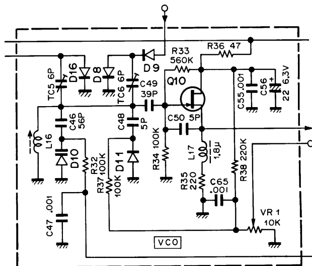
Fig. 6 VCO circuit
