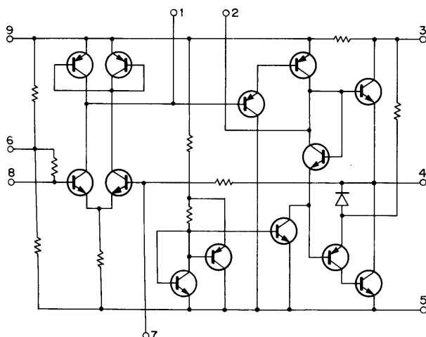
Fig. 2 BA526 Equivalent circuit (RX unit Q8)
