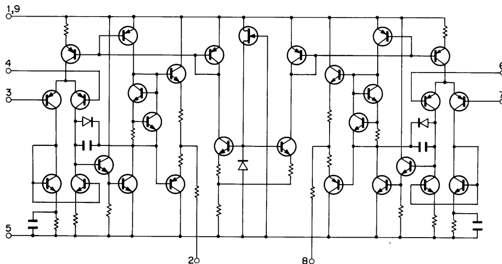
Fig. 5 LA6458S Equivalent circuit (TX unit IC2)
