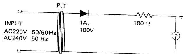
BC-2 SCHEMATIC DIAGRAM
