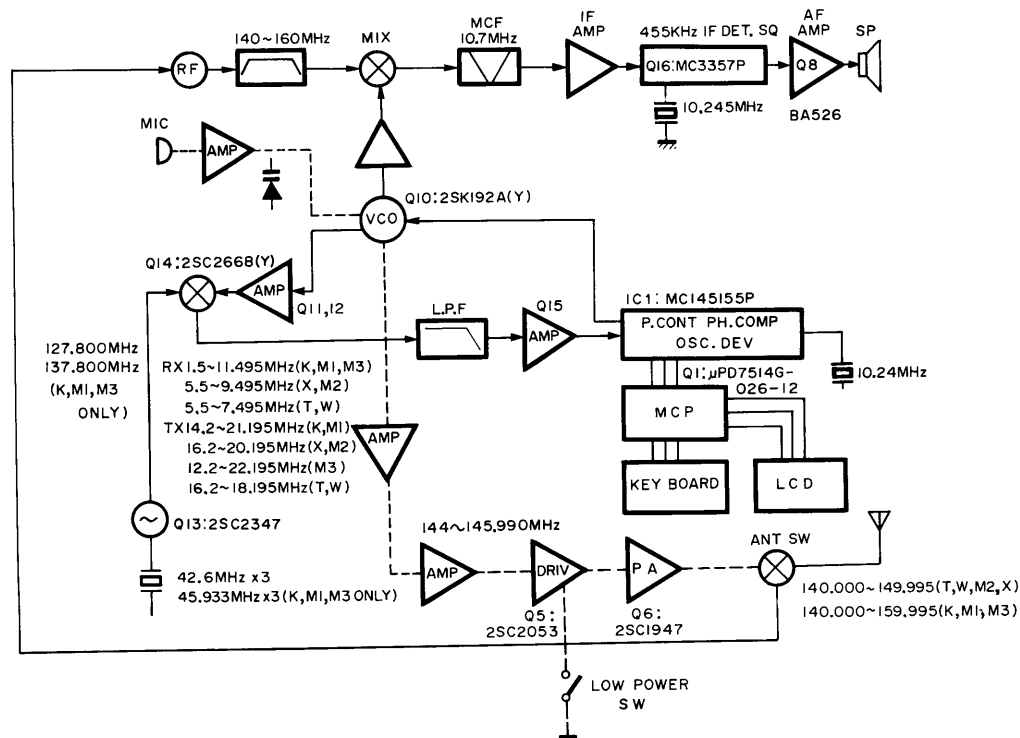
Fig. 15 Frequency-related block diagram
